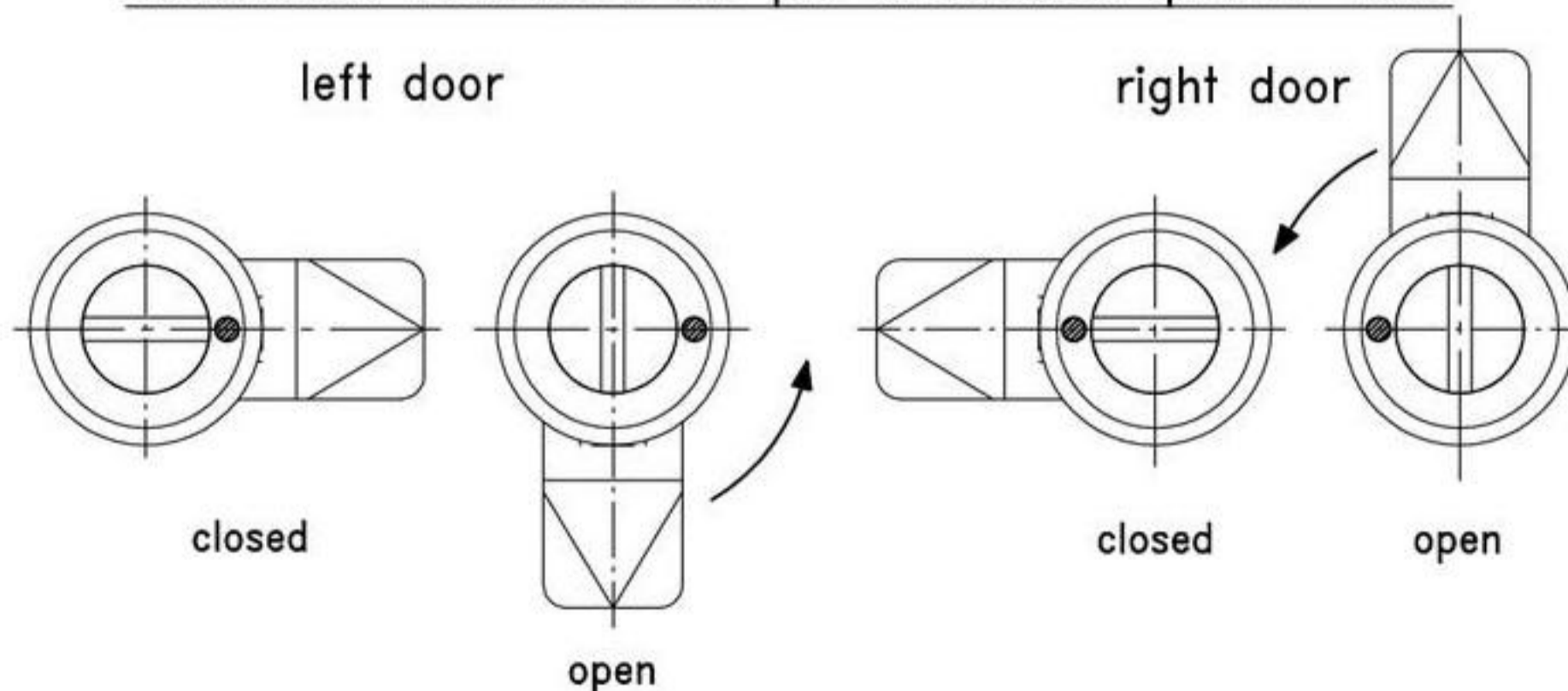
installation instruction for pre-assembled quarter-turn
