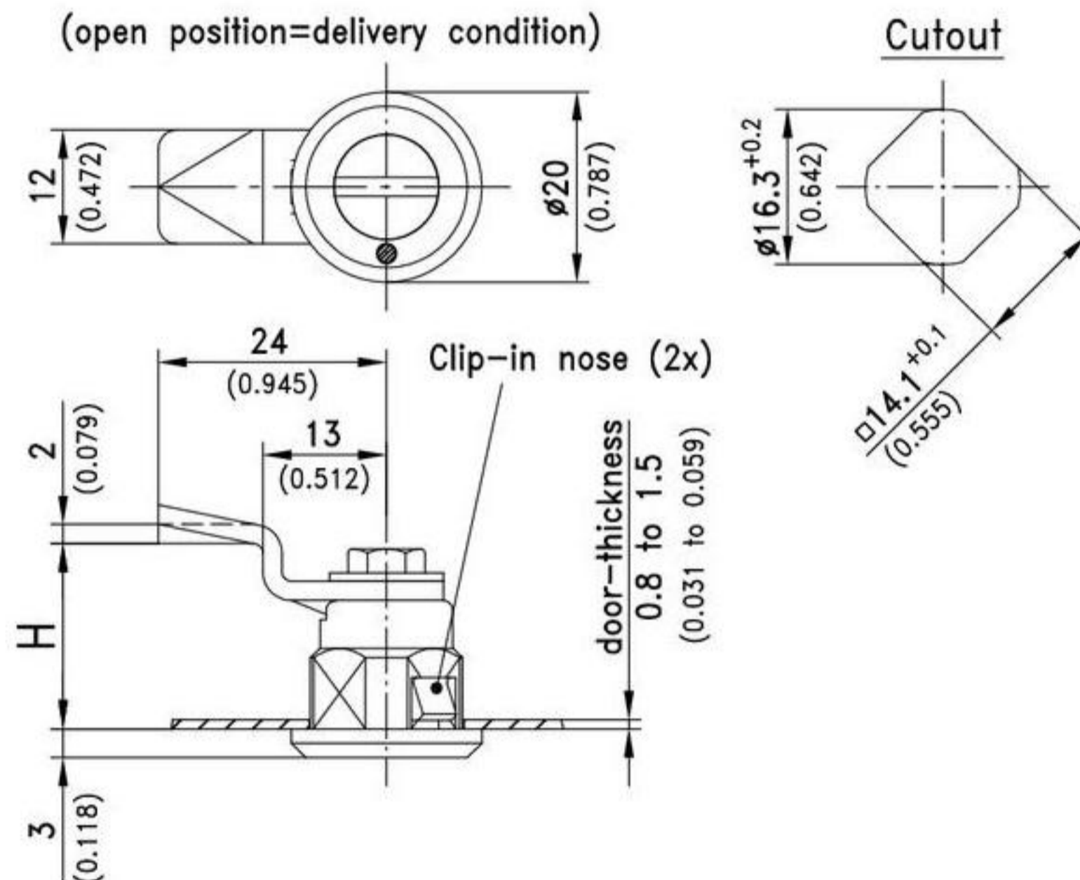
installation instruction for pre-assembled quarter-turn
