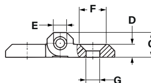
Countersunk version
