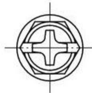
Phillips/slot version
