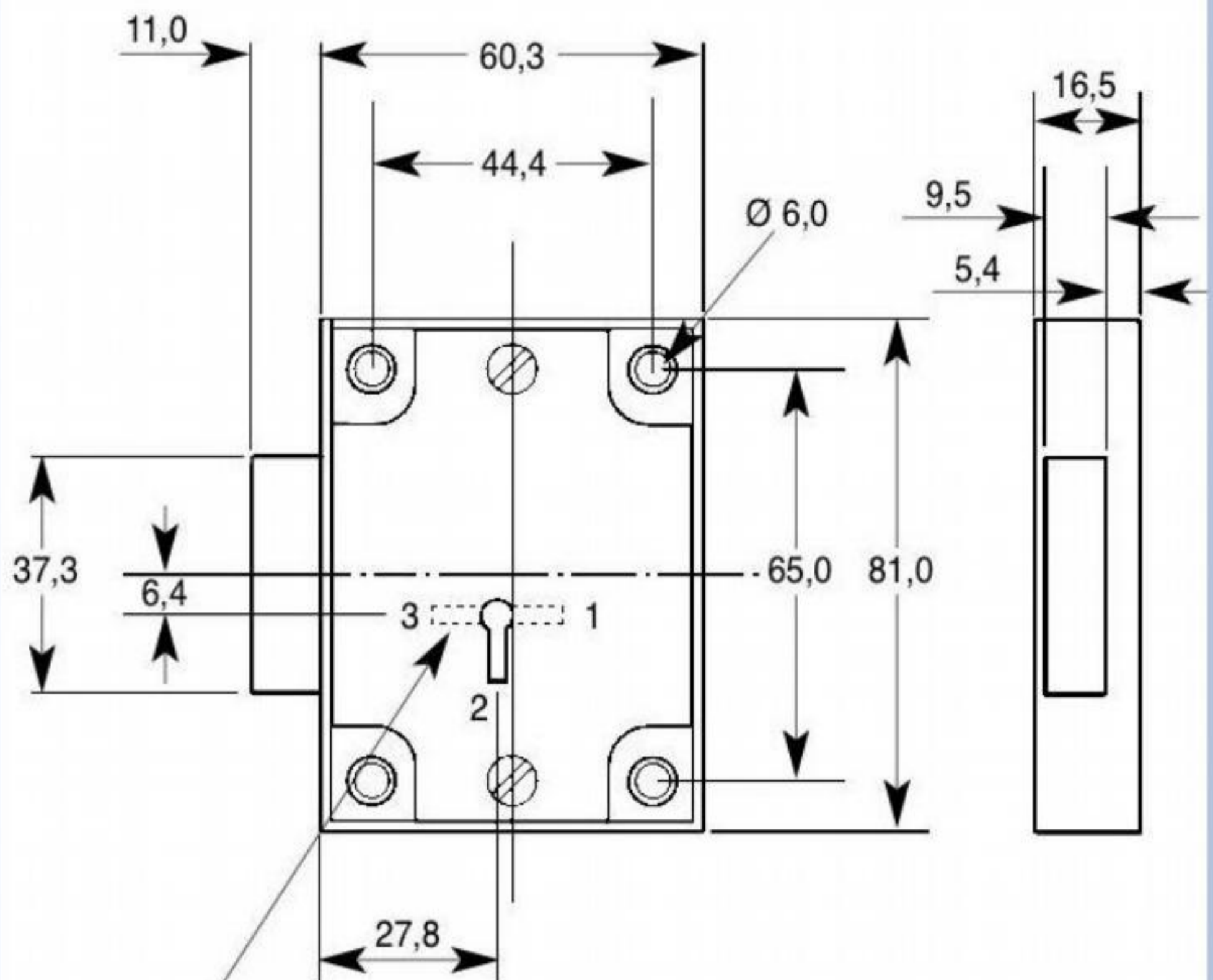
ALTERNATIVE KEYHOLE POSITIONS
