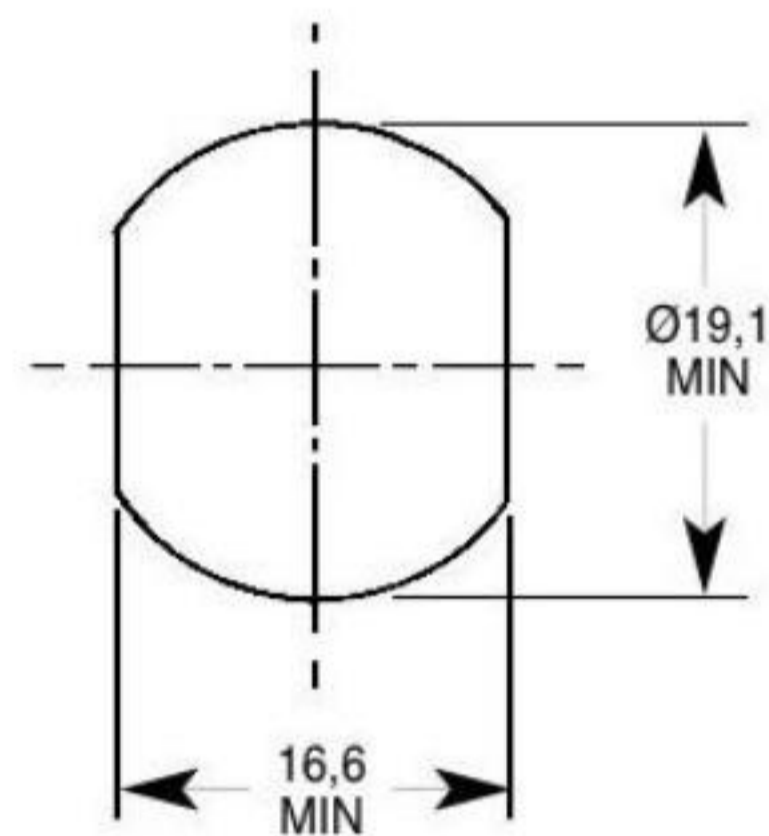
FIXING HOLE SIZE
